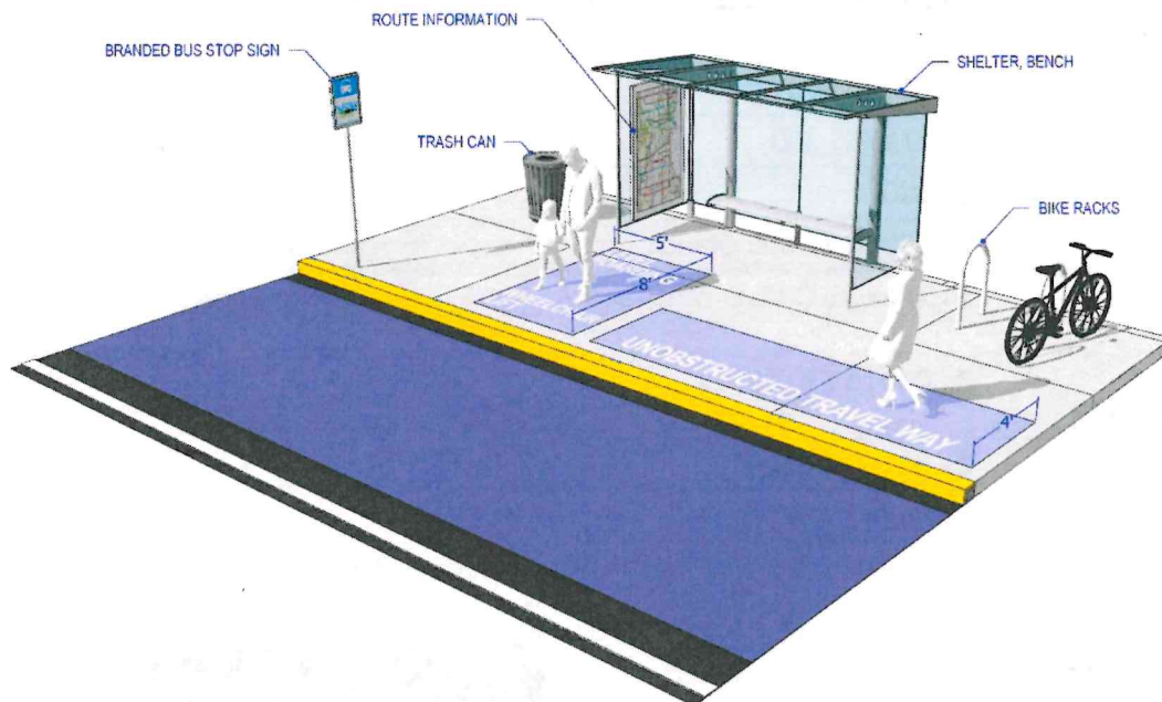
Figure 25. Typical Bus Stop Layout with Enhanced Amenities
